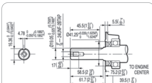
Albero - Shaft Mod.T/Q \varnothing 19,05 mm
